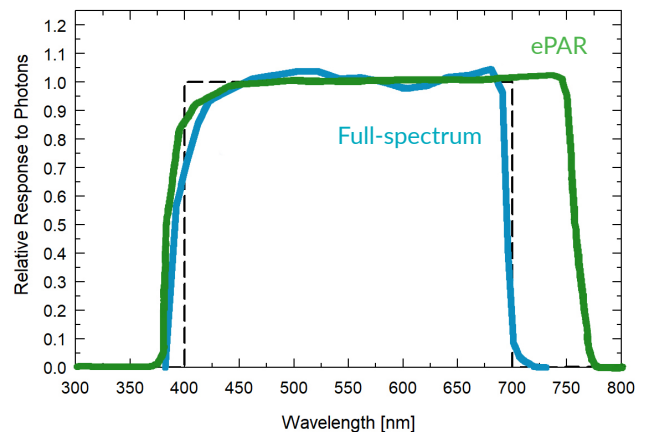
Spectral response of the SM-500 PAR sensor (blue) and SM-600 ePAR sensor (green) compared to the traditional PAR response (dashed).
