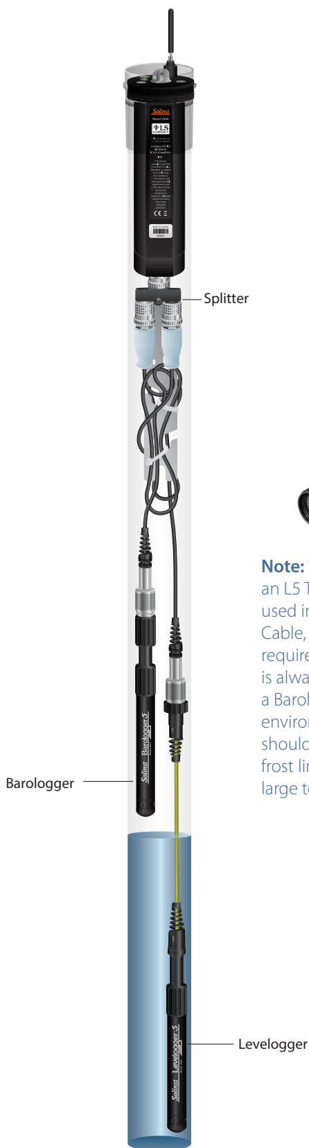
Figure 6-11 Levellogger and Barologger Installation (Reader Cable Connections Staggered)
